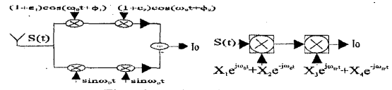
Fig. 12 IRR analysis model.
