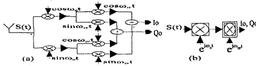
Fig. 11 Image-reject mixer architecture.
