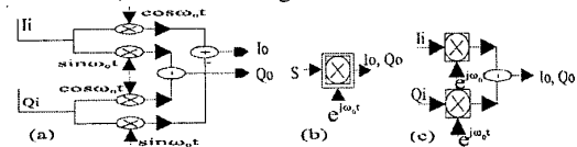
Fig. 6 Double_complex_mixer-LO (symbols).
