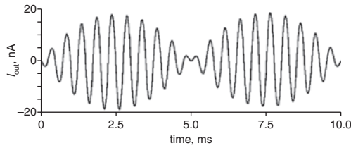
Fig. 3 Transient response of multiplier
