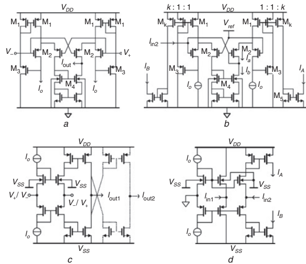
Fig. 2 Circuit building blocks
