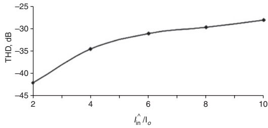
Fig. 4 Simulated THD against input signal amplitude, I_{in2} = 5 nA
