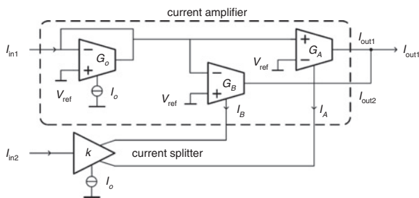
Fig. 1 Current multiplier block diagram
