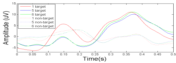
Fig. 3. Averages of target and non-target trials of Subject 4 at Cz
