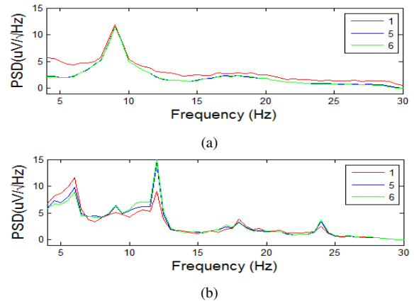
Fig. 2. a. Spectrum of eyes closed data of Subject 3 at Cz b. Spectrum of SSVEP seated data of Subject 8 at Cz
