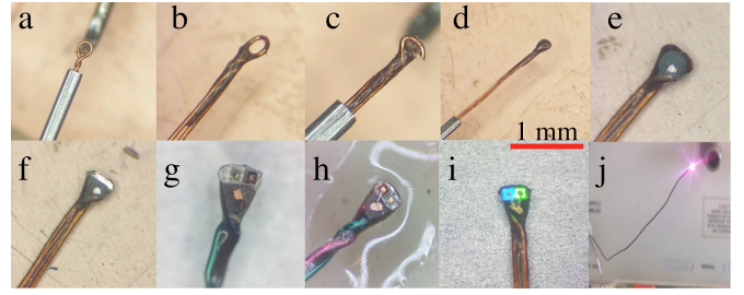
Fig. 6. Fully-flexible optrode fabrication procedure: a) A tiny loop of wire ( 80\ \mu\text{m} , 100\ \mu\text{m} , or 160\ \mu\text{m} in diameter), twist the wire ends. b) Apply a micro-drop of two-component glue on the twisted knot. c) Cut the loop open near the lower wire and shape it flat. d) Cover the open loop with two-component glue. e) and f) Cut pieces of glue and wire isolation in two steps. Here we create a copper dot and a copper line. g) Mount the bare dies of \mu LED on the copper line. h) Gold-bond the \mu LEDs gold plate to the copper dot. i) Test the \mu LEDs blinking and cover the top of the optrode with UV-curing glue. j) Fully-flexible optogenetics optrode.
