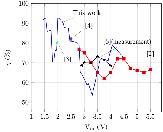
Fig. 6. Efficiency results of the RSC converter for various input voltages and V_{out} = 1\text{ V} . For [3] and [4] only the peak value has been considered.
