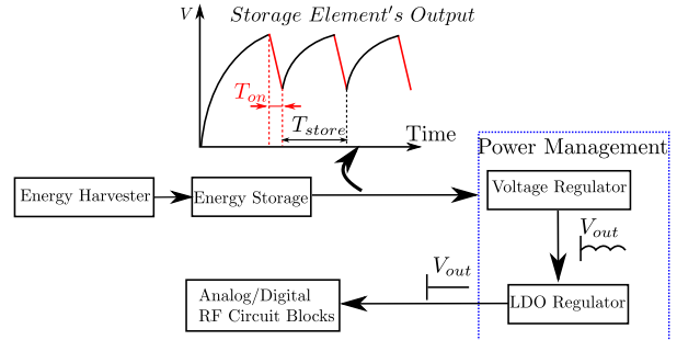
Fig. 1. Block diagram of a typical power management system.
