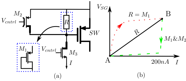
Fig. 5. (a) Schematic of the P-MOS switch implemented (b) with its equivalent resistance diagram in case a linear resistor, R (solid black line), or a diode-connected transistor, M_1 (dotted red line) is used. M_1 used in combination with M_2 allows for a fast turn-off of the main switch (green dashed line).
