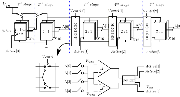
Fig. 4. Diagram of the RSC converter implemented and control.
