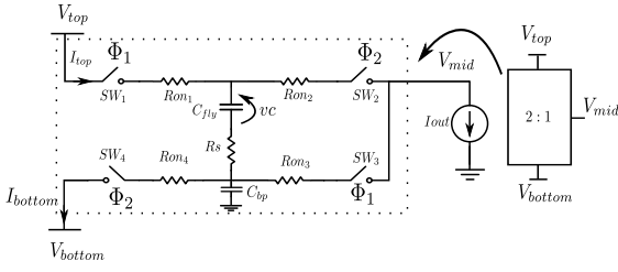
Fig. 2. Circuit representation of a 2 : 1 SC converter
