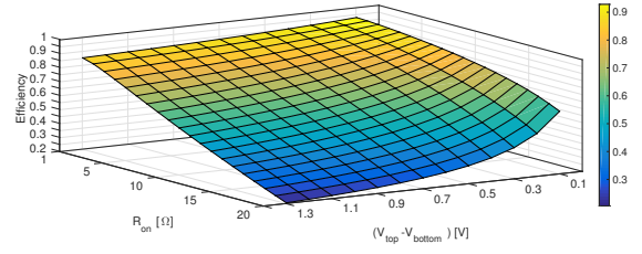
Fig. 3. Power efficiency for different on-resistances with C_{bp} = 5\%C_{fly} . V_{top} = 2.2 V, while V_{bottom} has been swapped from 2.1 V to 0.9 V.
